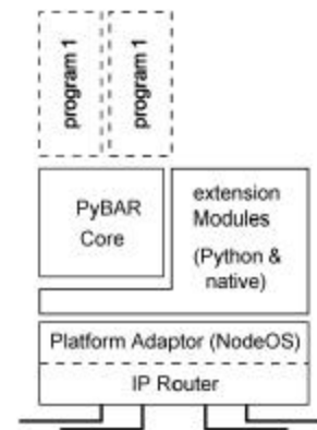
Figure 12 : Python Based Active Router
