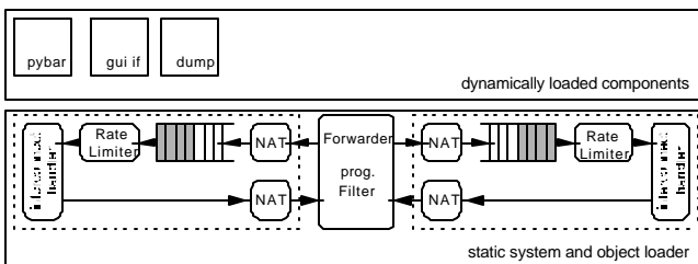
Figure 3 : Virtual Router Implementation Architecture
