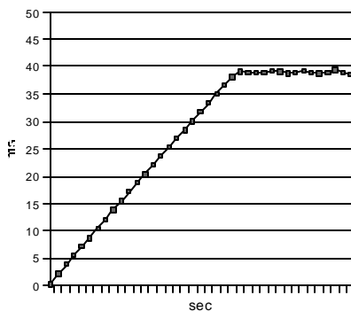
Figure 5 : Delay of a virtual router FIFO queue using a 4 Mbps link
