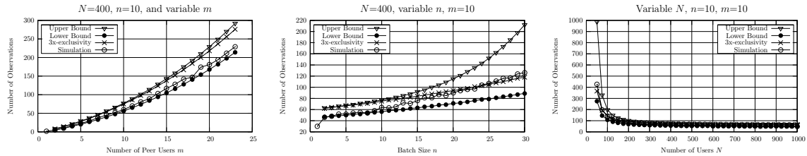
Figure 5. Number of observation required for Case (b)
