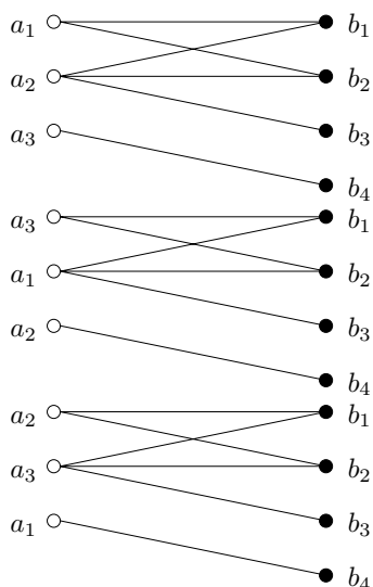
Figure 3. Permutation of nodes in bipartite graph.
