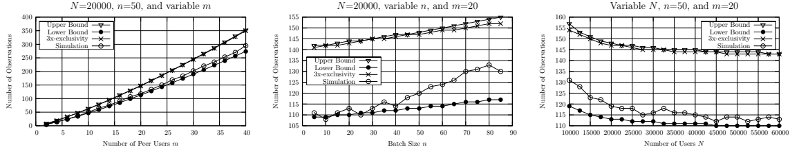
Figure 4. Number of observation required for Case (a)
