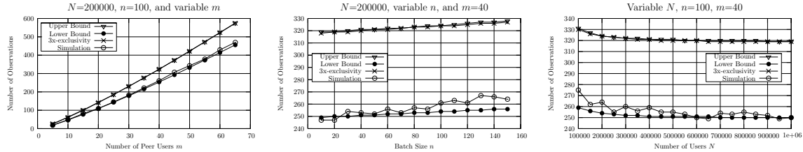
Figure 6. Number of observation required for Case (c)
